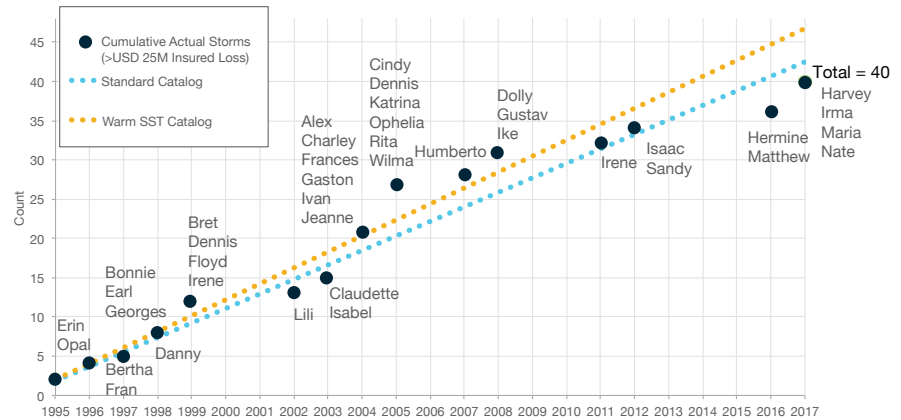
Figure 2. Observed cumulative count of loss-causing storms (>USD 25 million insured loss) from 1995 to the present, shown with the cumulative frequency of these storms implemented in AIR's standard and WSST catalogs. Note that both landfalling and bypassing storms are included in this analysis, and modeled historical losses are based on today's exposures. (Source: AIR)
