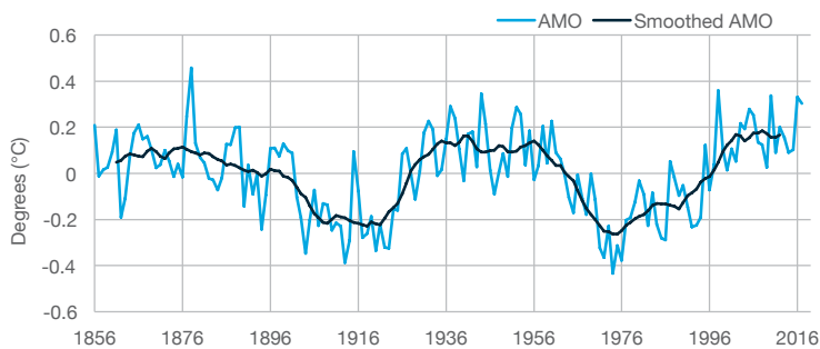
Figure 1. Annual average and smoothed average of the Atlantic Multidecadal Oscillation (Data Source: NOAA Earth System Research Laboratory)
